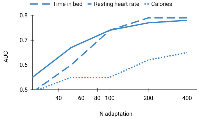
Figure 2: Comparison of models trained with three different self-supervised objective tasks. The AUC (y-axis) quantifies the performance on the adaptation task, ILI prediction.
